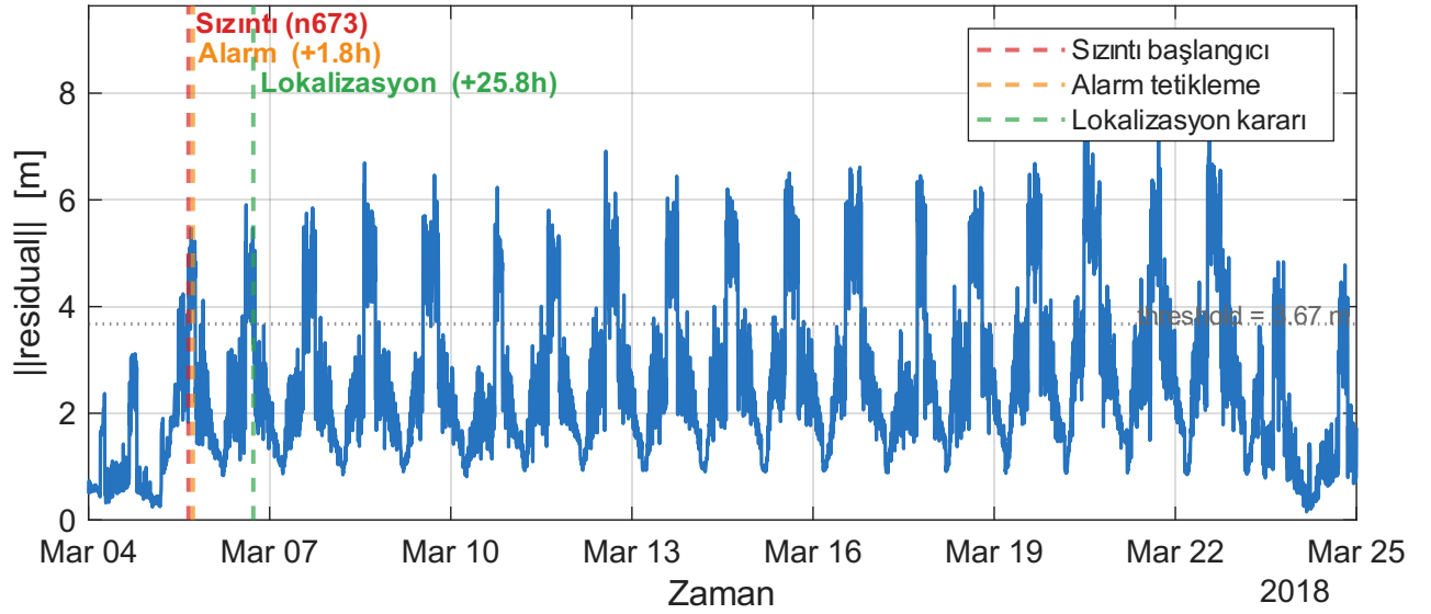
Plan C — Residual norm ve real-time alarm
